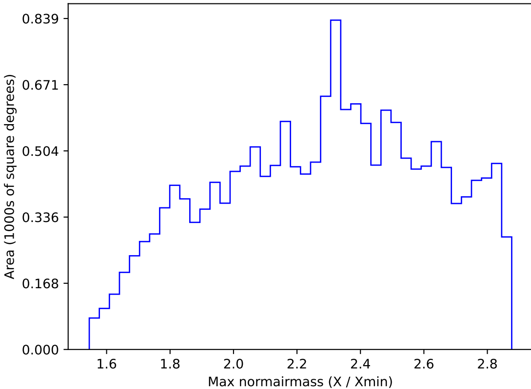
scp_reweight_v3.3_10yrs WFD i band: Max normairmass
