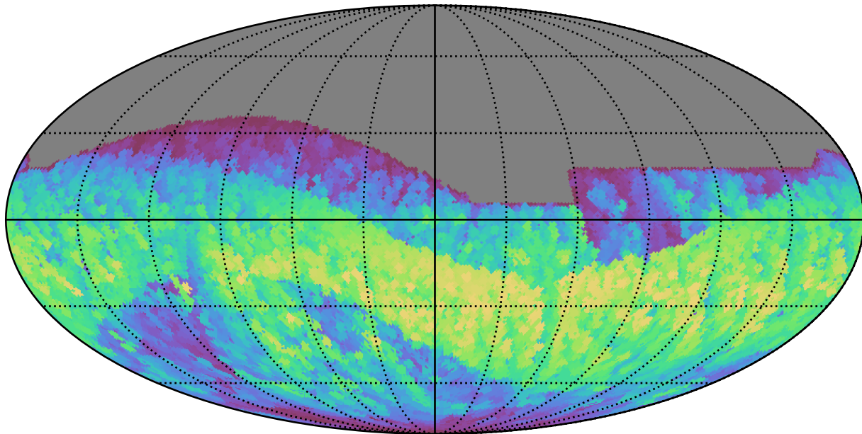
scp_reweight_v3.3_10yrs All sky z band: Max normairmass
