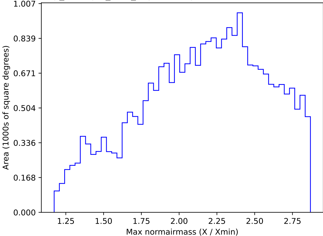
scp_reweight_v3.3_10yrs All sky z band: Max normairmass
