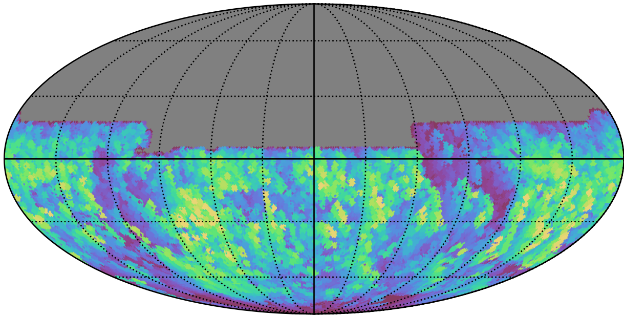
scp_reweight_v3.3_10yrs All sky y band: Max normairmass
