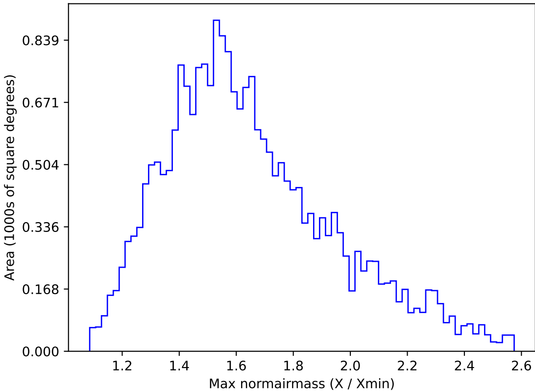
scp_reweight_v3.3_10yrs All sky u band: Max normairmass
