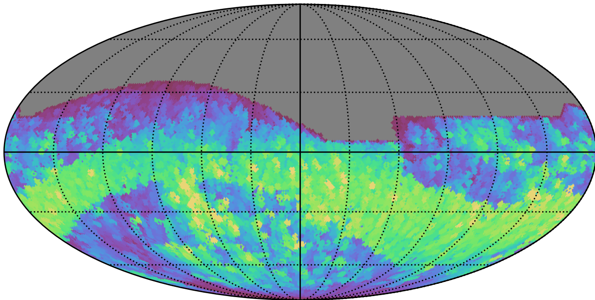
scp_reweight_v3.3_10yrs All sky r band: Max normairmass
