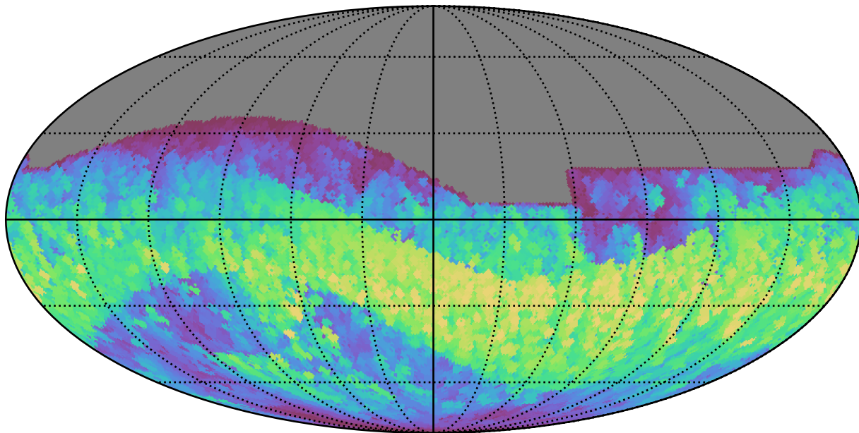
scp_reweight_v3.3_10yrs All sky i band: Max normairmass
