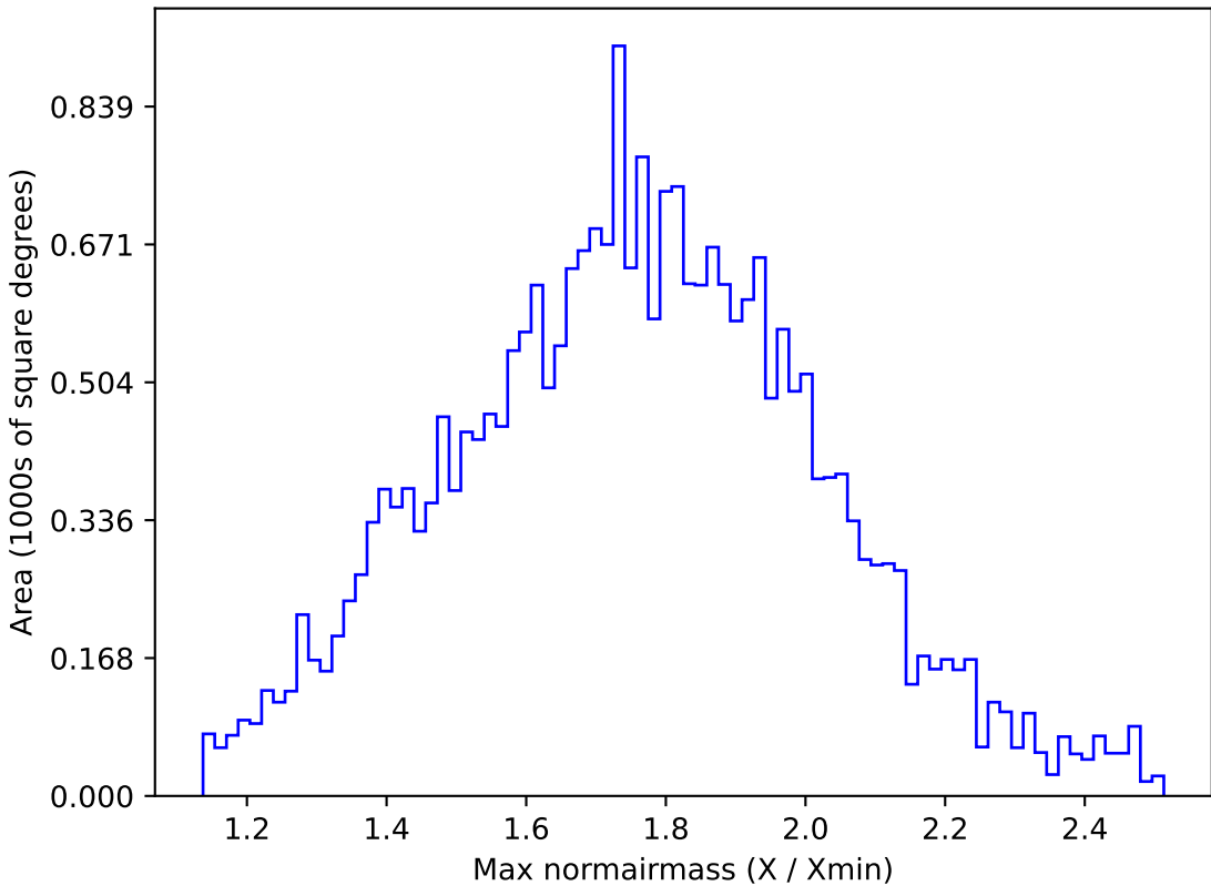
scp_reweight_v3.3_10yrs All sky g band: Max normairmass
