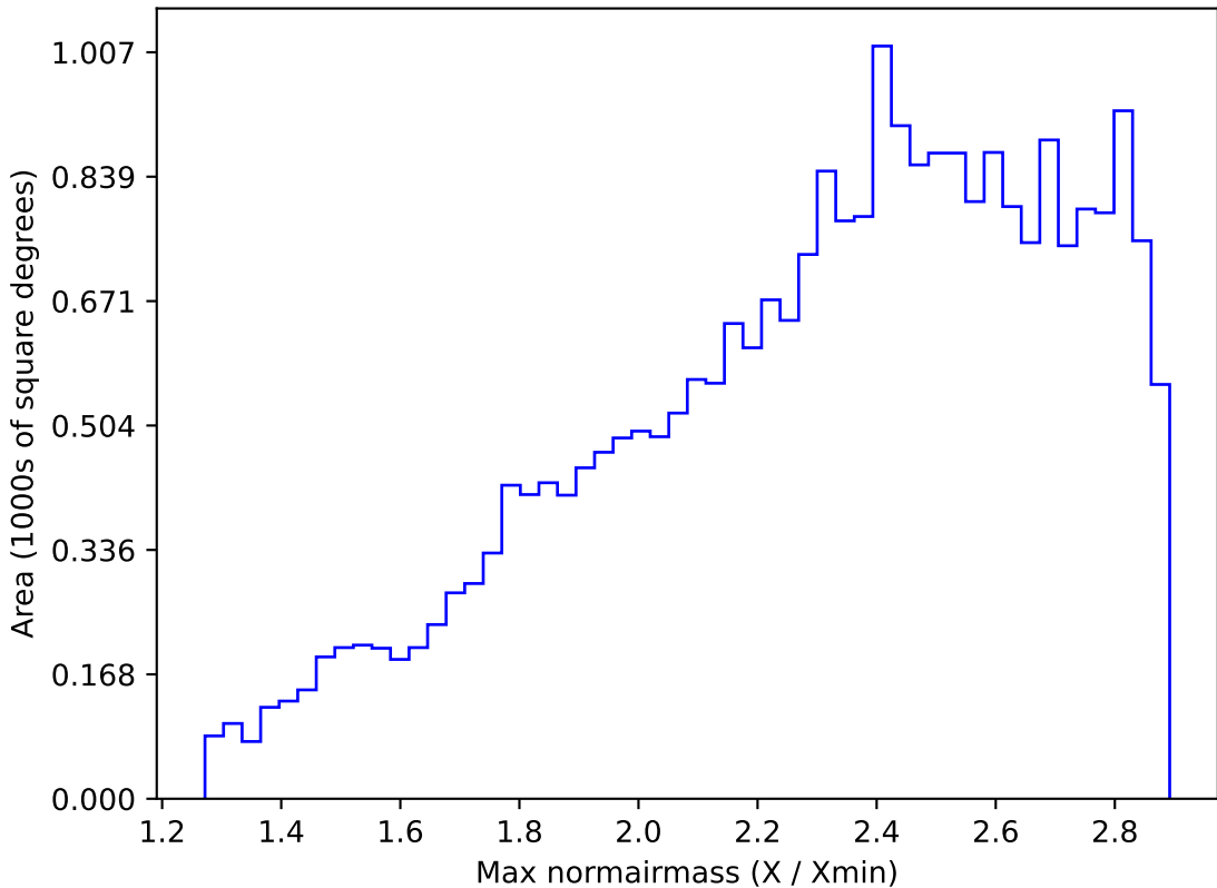
scp_reweight_v3.3_10yrs All sky all bands: Max normairmass
