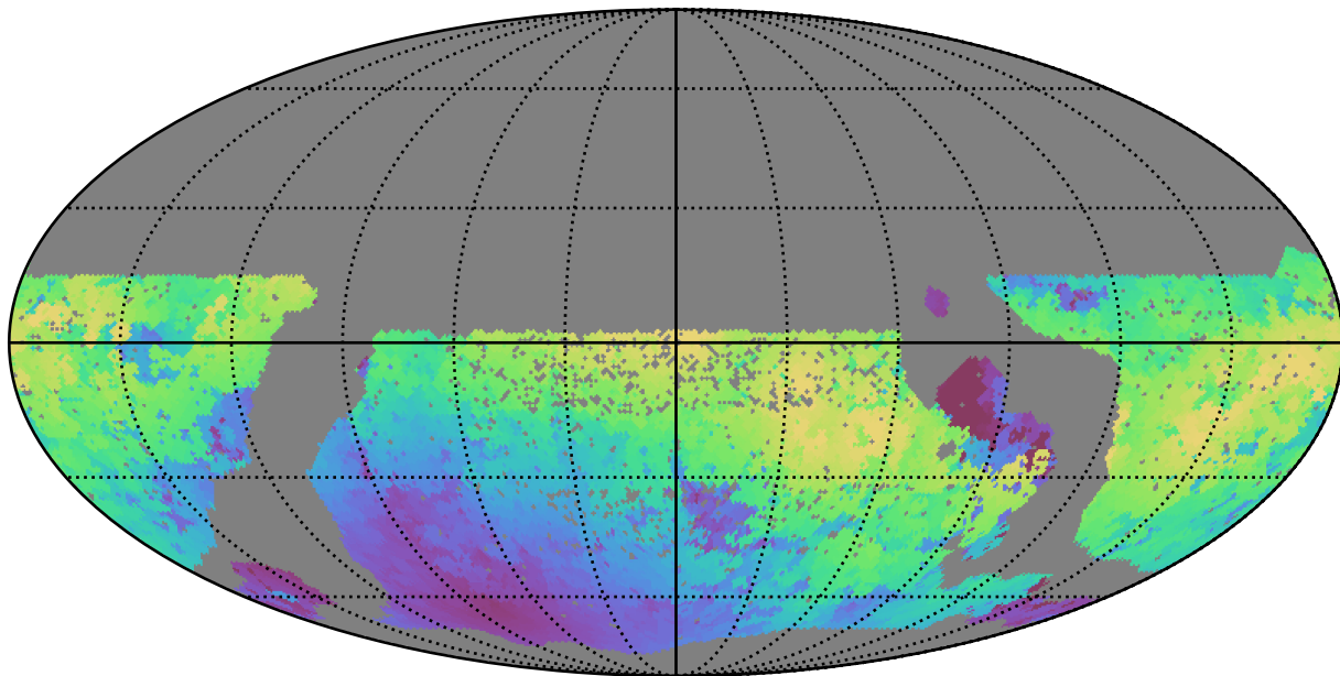
scp_reweight_v3.3_10yrs WFD y band: Max moonDistance
