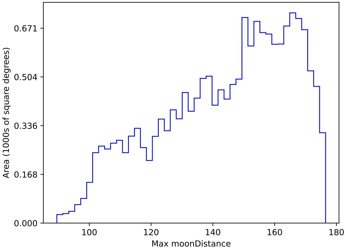
scp_reweight_v3.3_10yrs WFD y band: Max moonDistance
