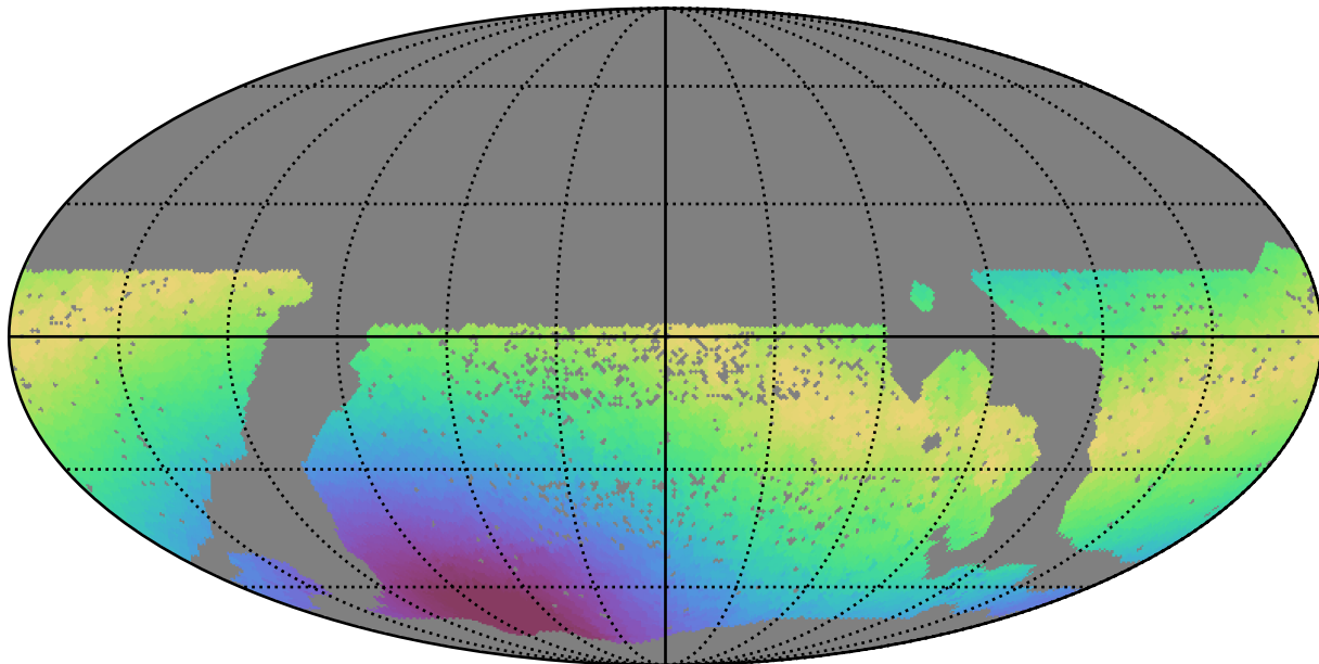
scp_reweight_v3.3_10yrs WFD u band: Max moonDistance
