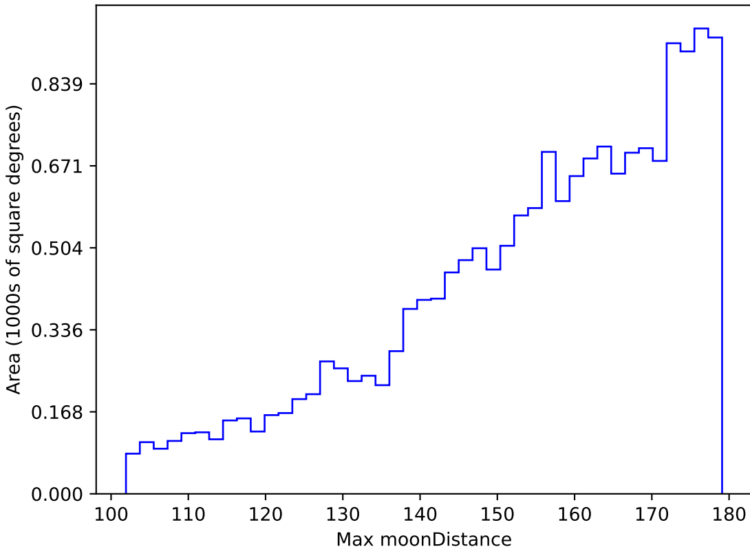
scp_reweight_v3.3_10yrs WFD u band: Max moonDistance
