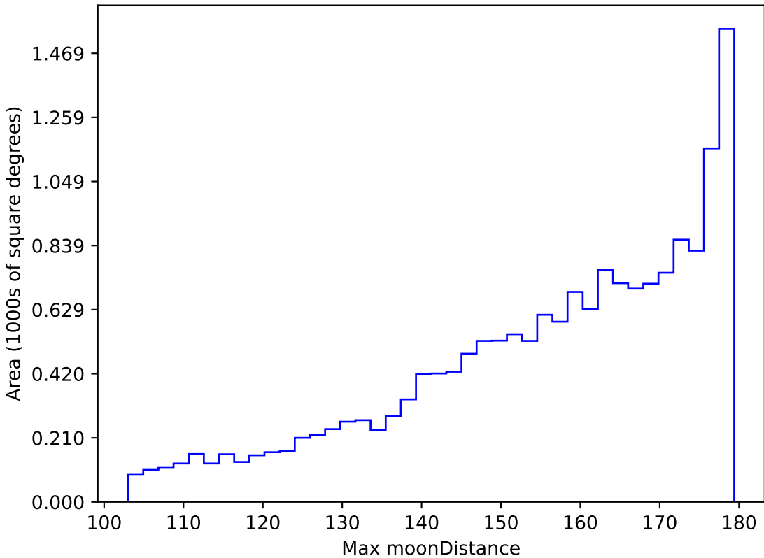
scp_reweight_v3.3_10yrs WFD r band: Max moonDistance
