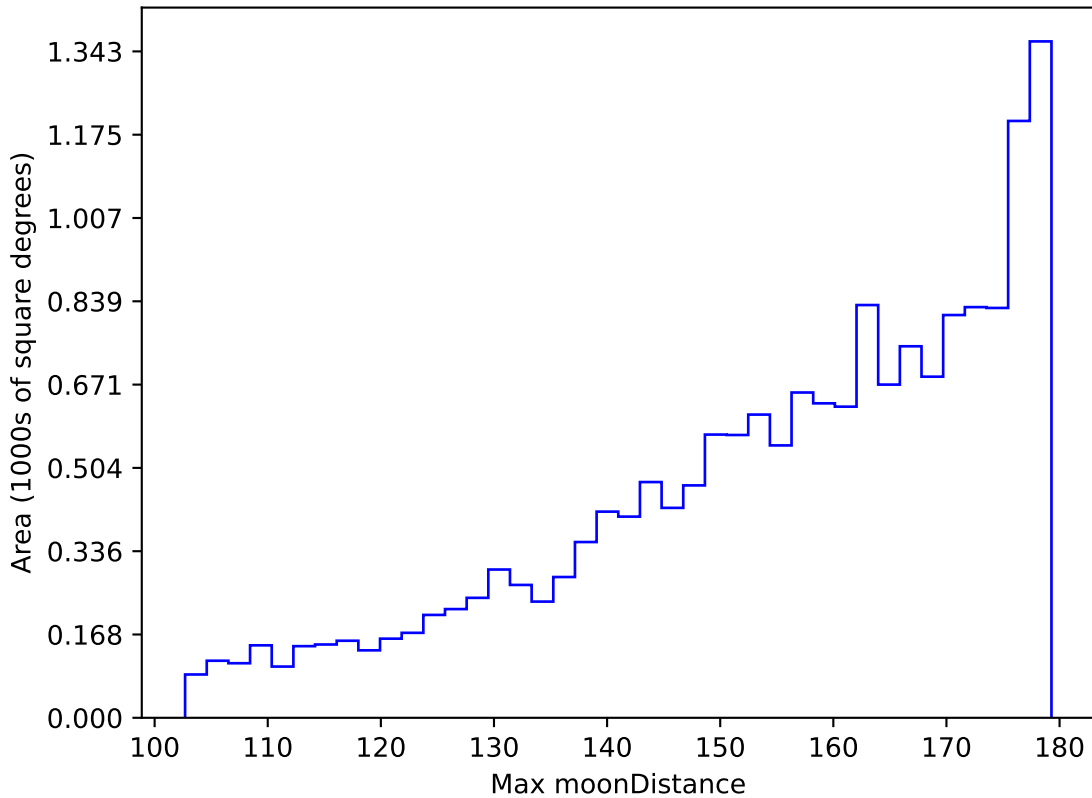
scp_reweight_v3.3_10yrs WFD i band: Max moonDistance
