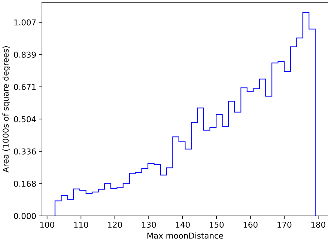
scp_reweight_v3.3_10yrs WFD g band: Max moonDistance
