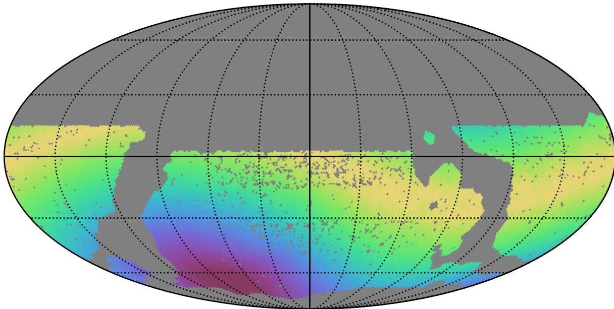
scp_reweight_v3.3_10yrs WFD all bands: Max moonDistance
