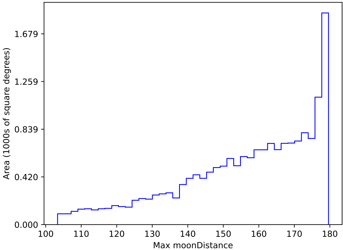
scp_reweight_v3.3_10yrs WFD all bands: Max moonDistance
