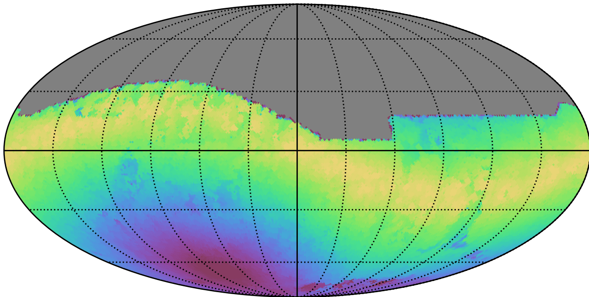
scp_reweight_v3.3_10yrs All sky z band: Max moonDistance
