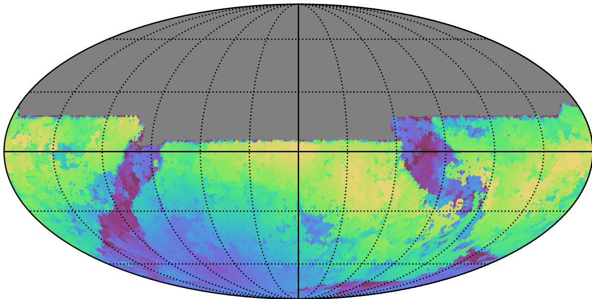
scp_reweight_v3.3_10yrs All sky y band: Max moonDistance
