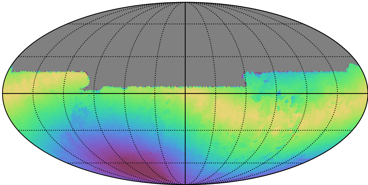
scp_reweight_v3.3_10yrs All sky u band: Max moonDistance
