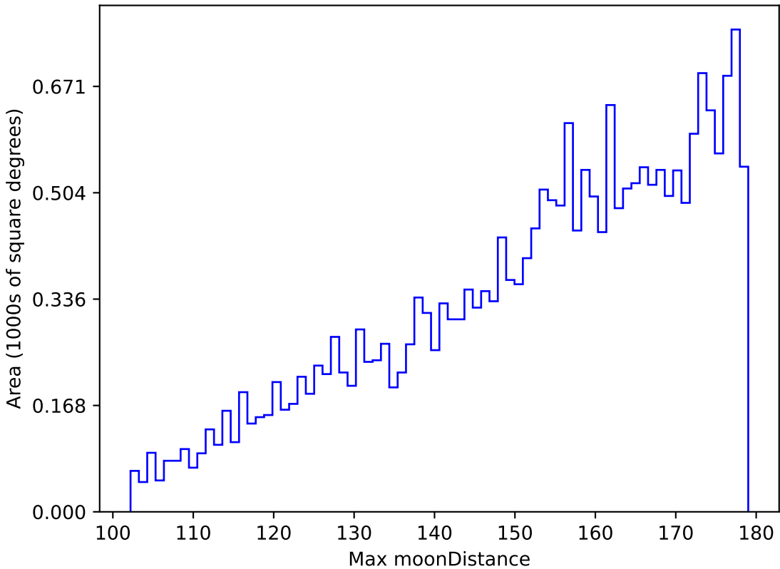
scp_reweight_v3.3_10yrs All sky u band: Max moonDistance
