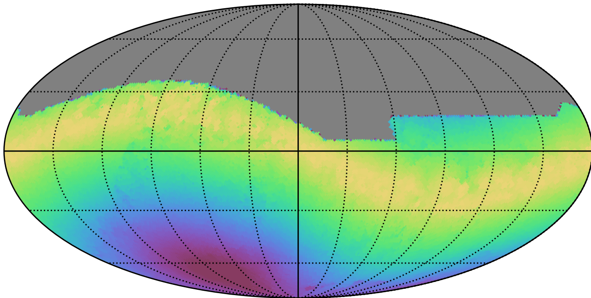
scp_reweight_v3.3_10yrs All sky r band: Max moonDistance
