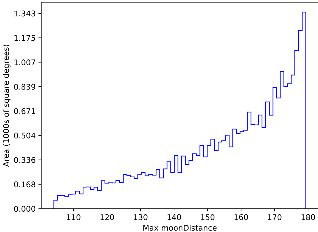
scp_reweight_v3.3_10yrs All sky r band: Max moonDistance
