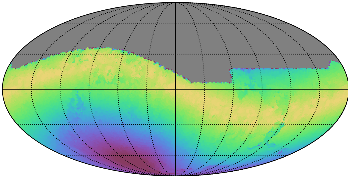
scp_reweight_v3.3_10yrs All sky i band: Max moonDistance
