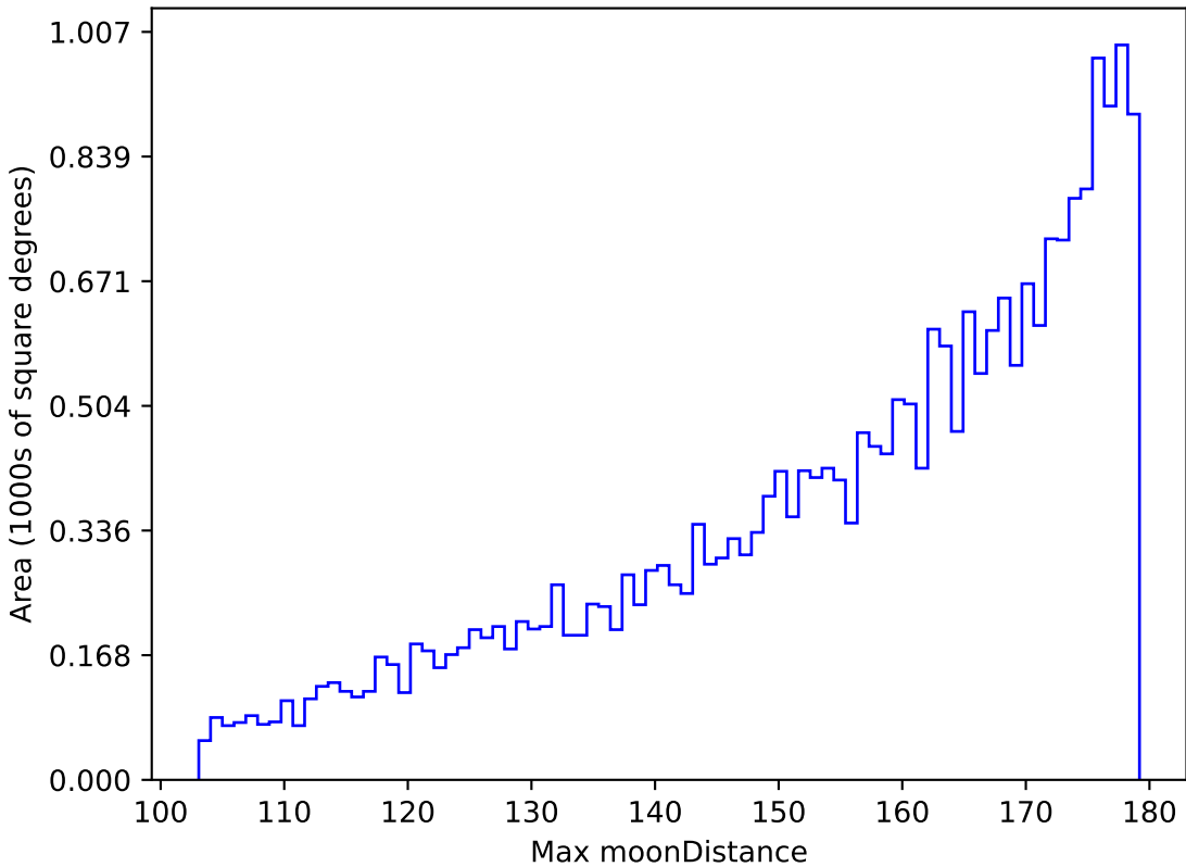
scp_reweight_v3.3_10yrs All sky i band: Max moonDistance
