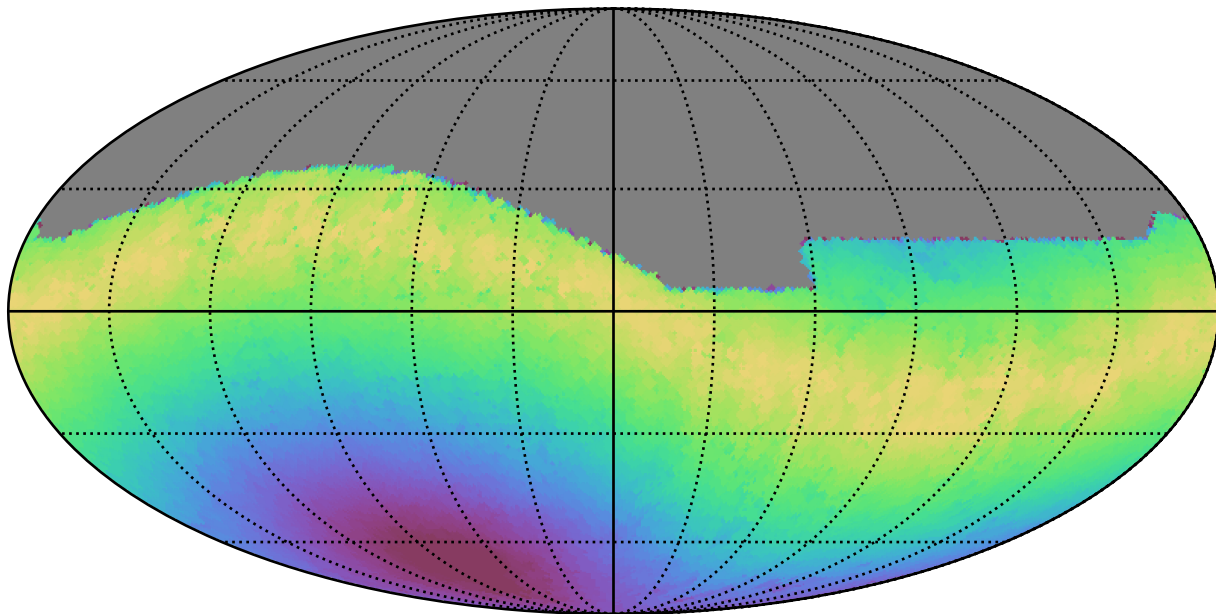
scp_reweight_v3.3_10yrs All sky g band: Max moonDistance
