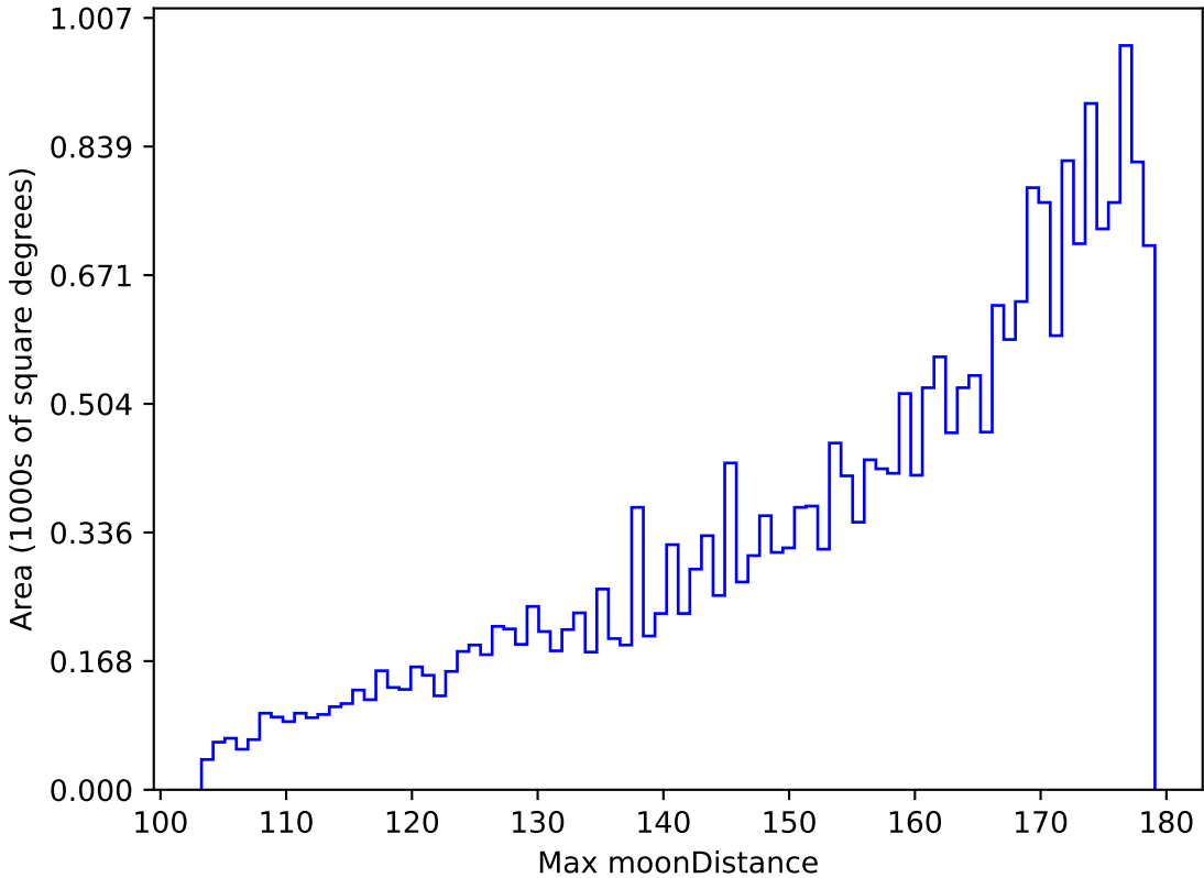
scp_reweight_v3.3_10yrs All sky g band: Max moonDistance
