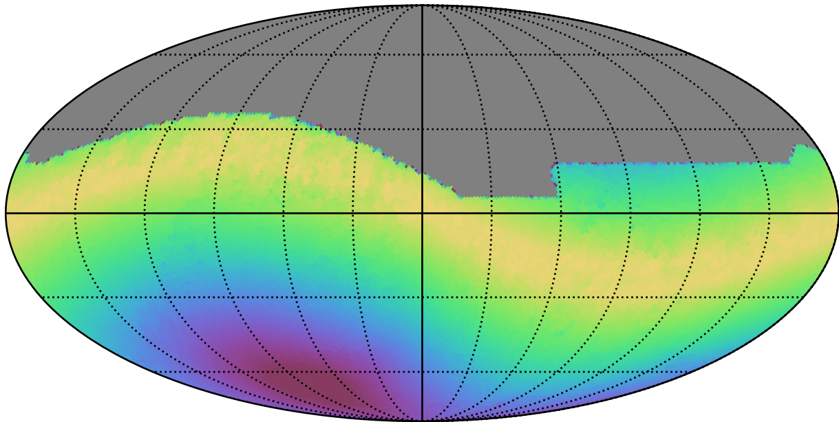
scp_reweight_v3.3_10yrs All sky all bands: Max moonDistance
