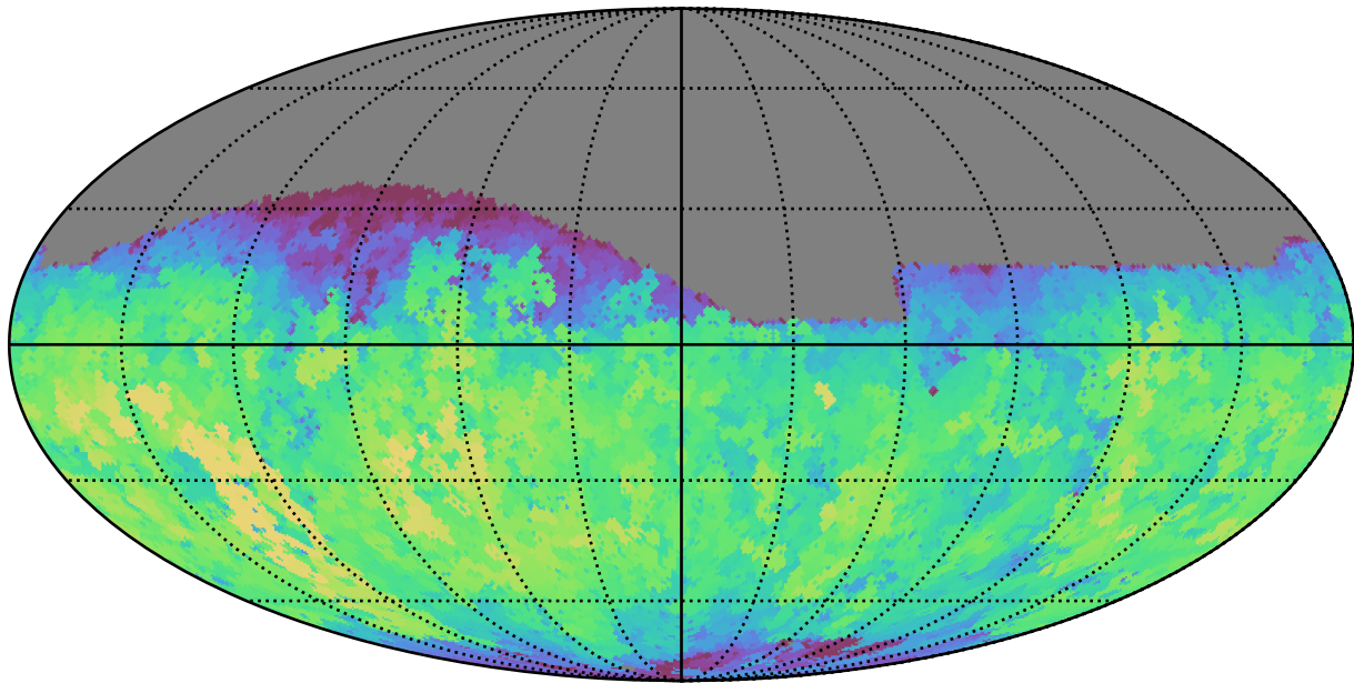
scp_reweight_v3.3_10yrs Yr 1 z band: Max fiveSigmaDepth
