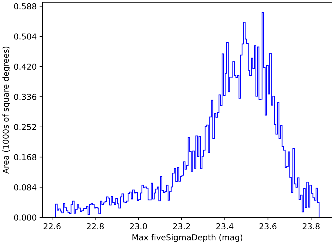
scp_reweight_v3.3_10yrs Yr 1 z band: Max fiveSigmaDepth
