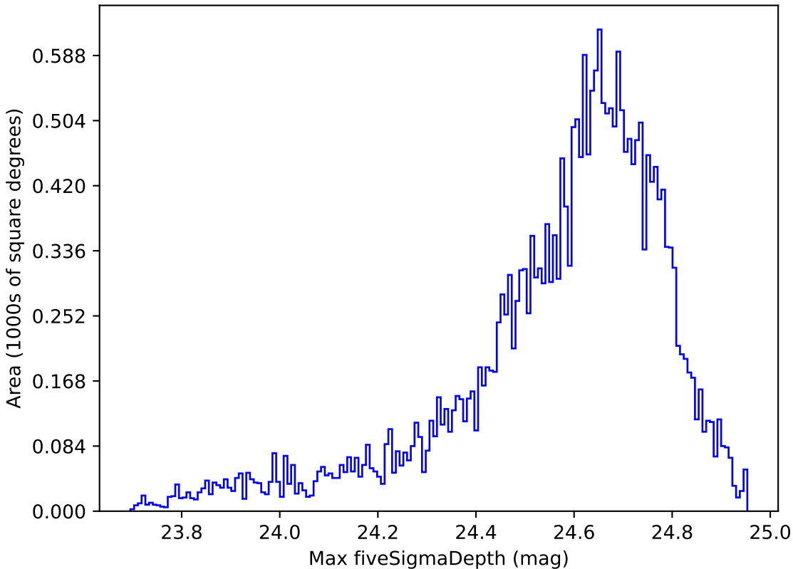
scp_reweight_v3.3_10yrs Yr 1 r band: Max fiveSigmaDepth
