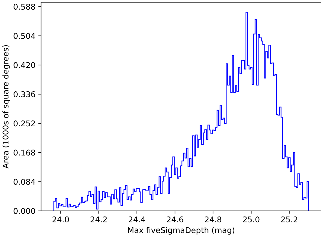
scp_reweight_v3.3_10yrs Yr 1 g band: Max fiveSigmaDepth
