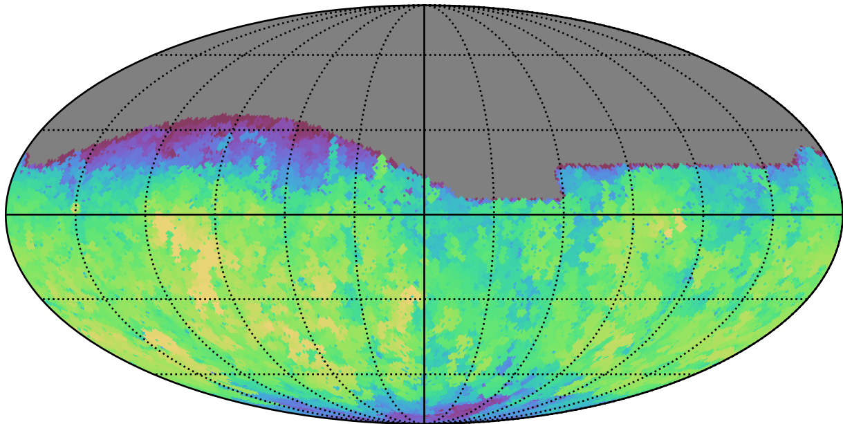
scp_reweight_v3.3_10yrs Yr 1 all bands: Max fiveSigmaDepth
