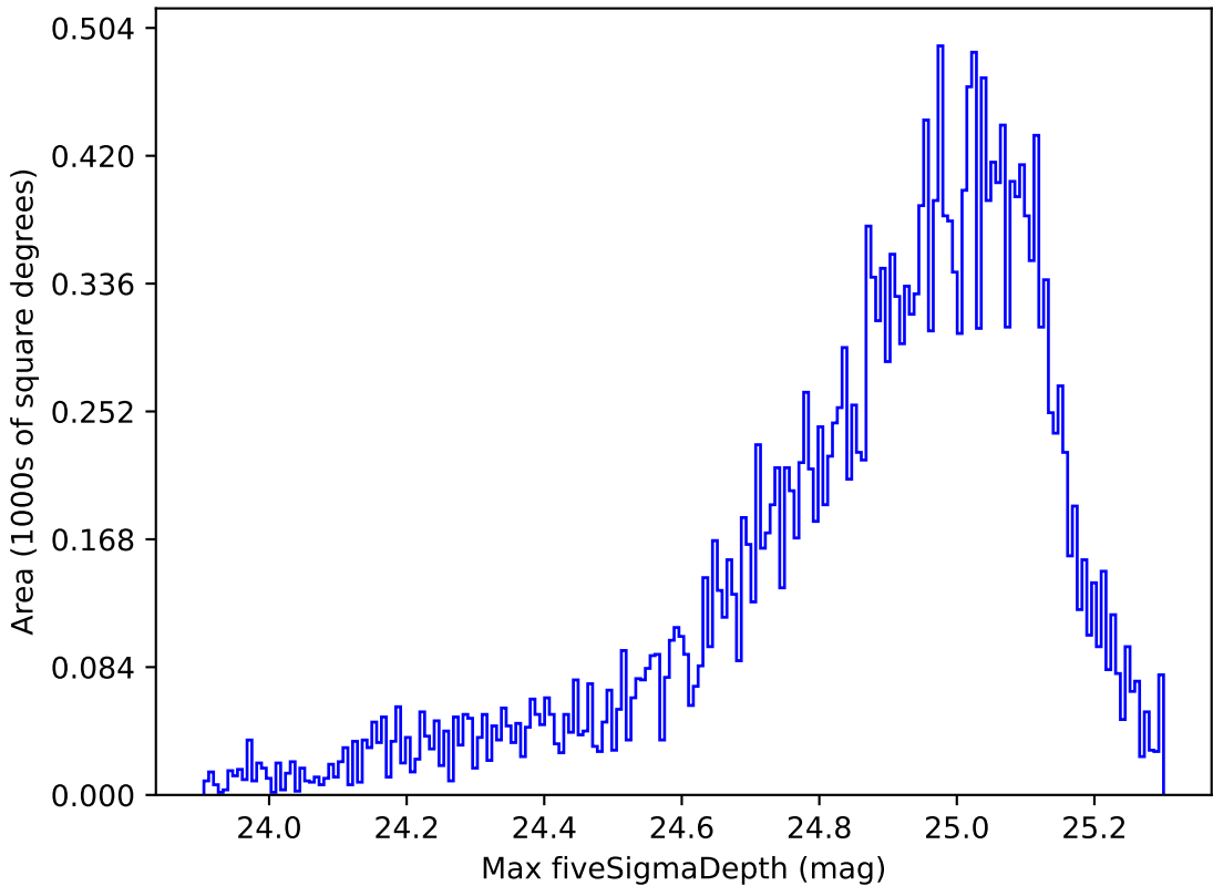
scp_reweight_v3.3_10yrs Yr 1 all bands: Max fiveSigmaDepth
