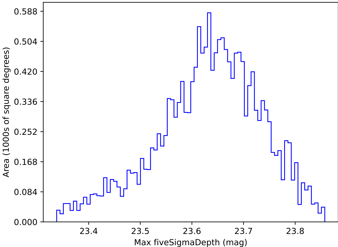
scp_reweight_v3.3_10yrs WFD z band: Max fiveSigmaDepth
