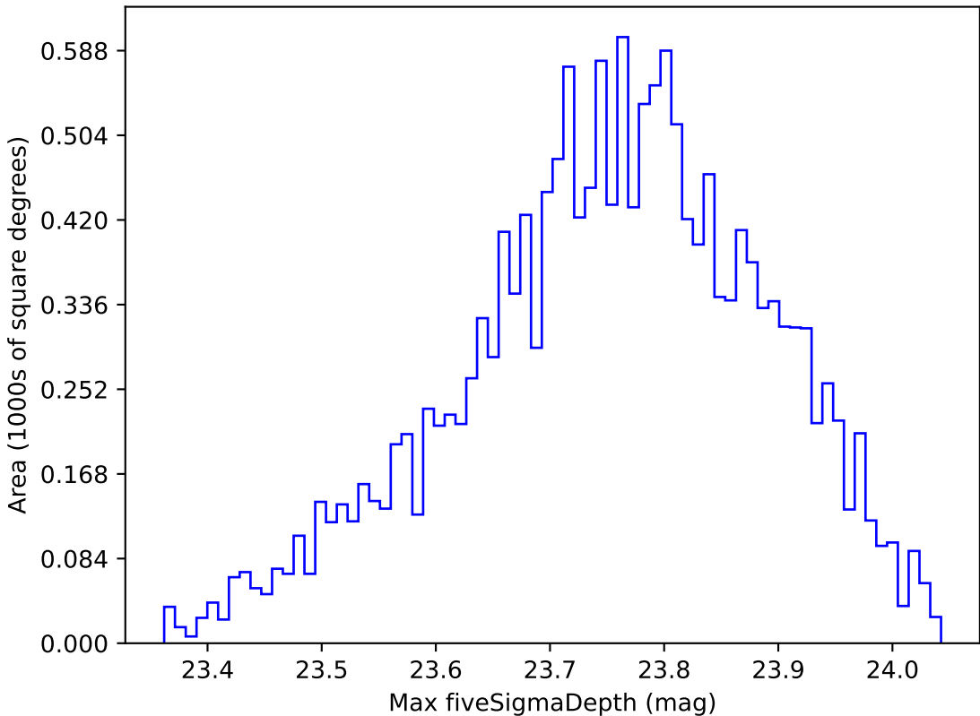
scp_reweight_v3.3_10yrs WFD u band: Max fiveSigmaDepth
