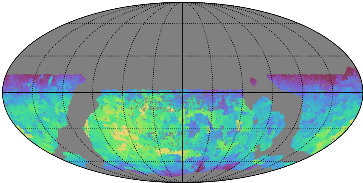
scp_reweight_v3.3_10yrs WFD r band: Max fiveSigmaDepth
