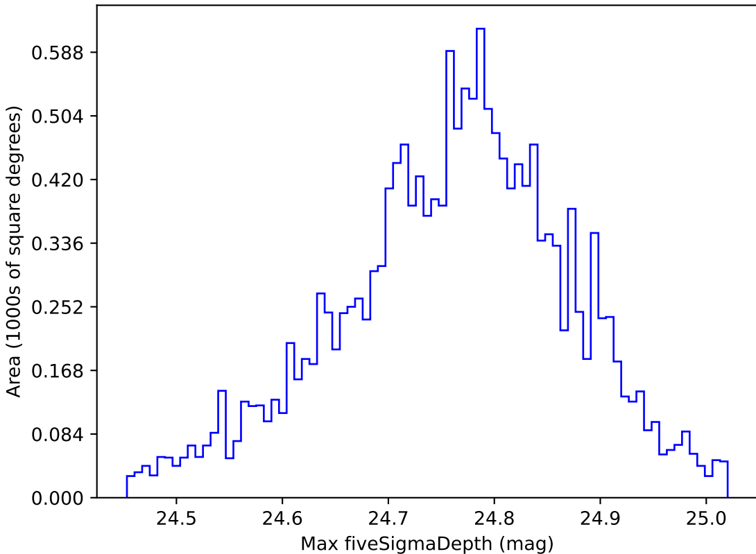
scp_reweight_v3.3_10yrs WFD r band: Max fiveSigmaDepth
