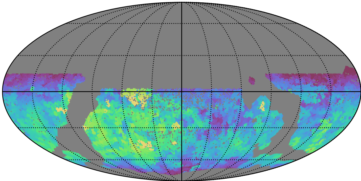
scp_reweight_v3.3_10yrs WFD g band: Max fiveSigmaDepth
