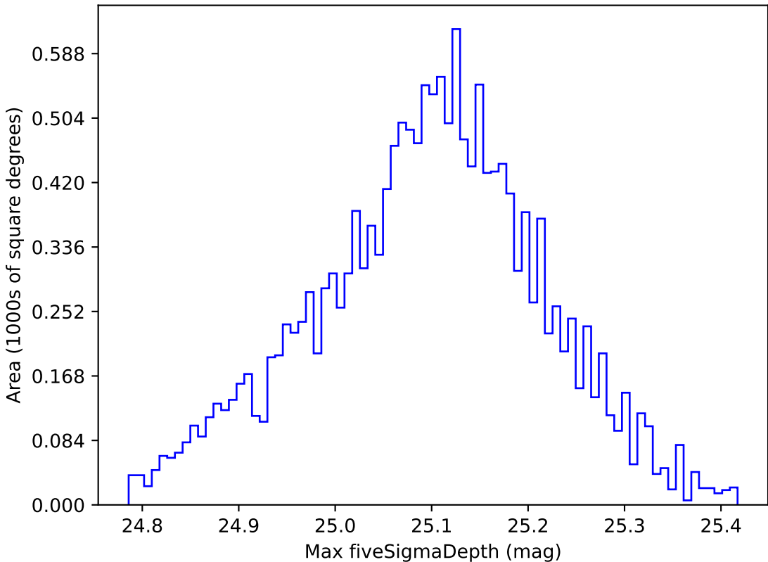
scp_reweight_v3.3_10yrs WFD all bands: Max fiveSigmaDepth
