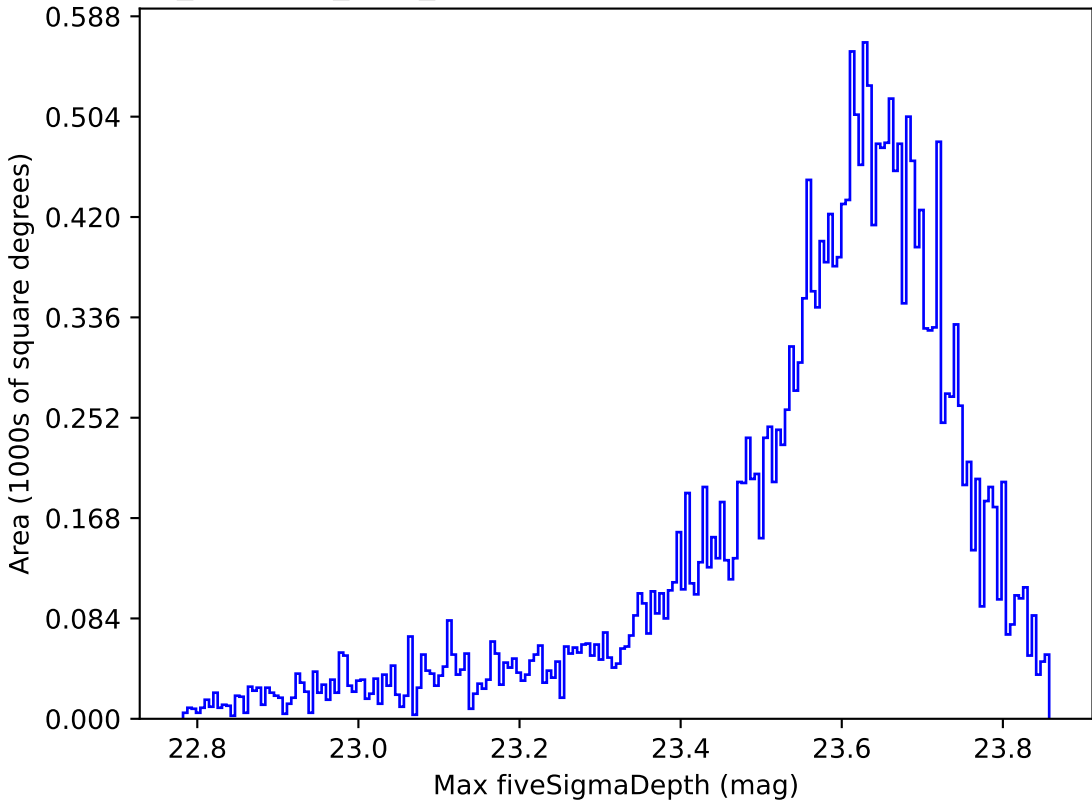
scp_reweight_v3.3_10yrs All sky z band: Max fiveSigmaDepth
