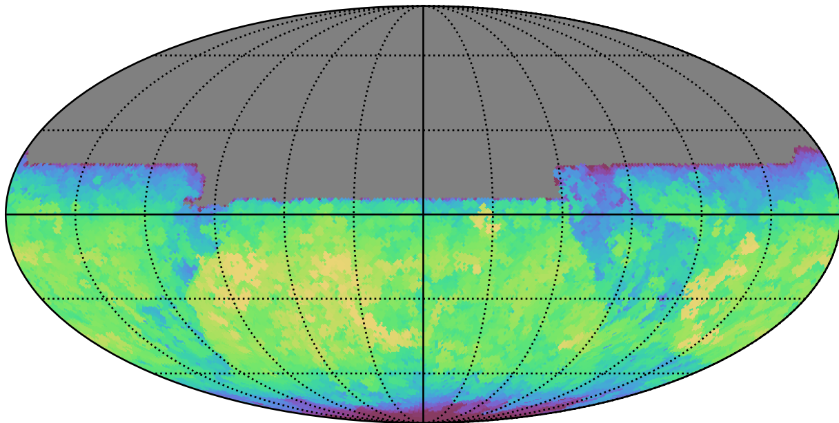
scp_reweight_v3.3_10yrs All sky y band: Max fiveSigmaDepth
