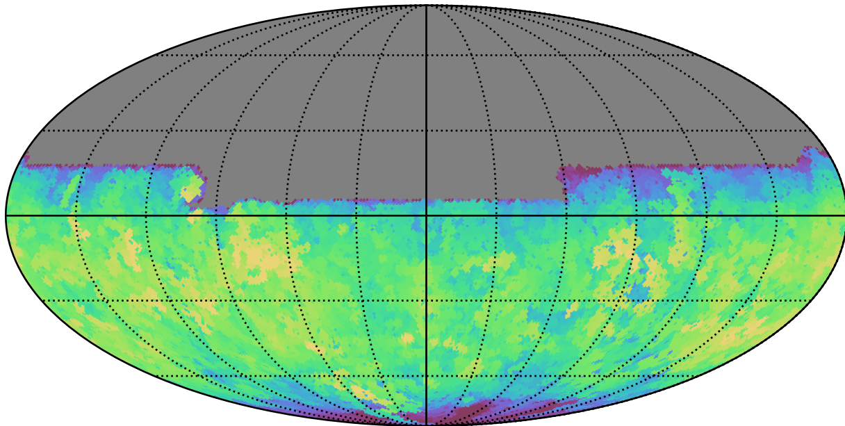
scp_reweight_v3.3_10yrs All sky u band: Max fiveSigmaDepth
