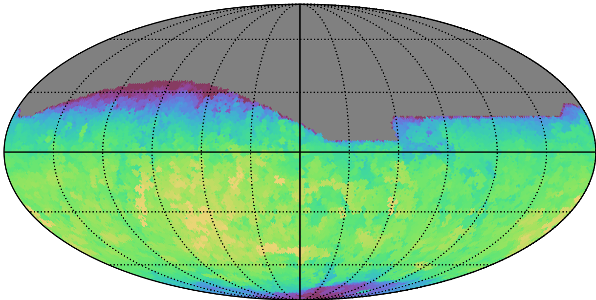
scp_reweight_v3.3_10yrs All sky r band: Max fiveSigmaDepth
