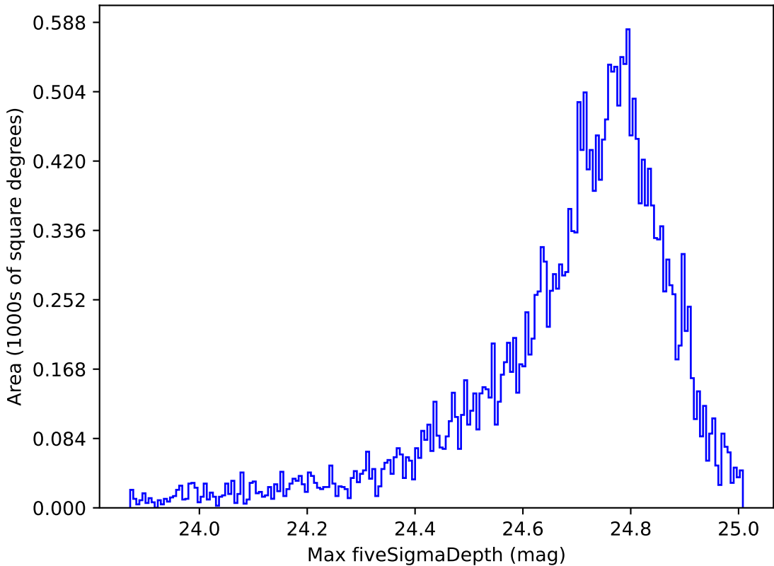
scp_reweight_v3.3_10yrs All sky r band: Max fiveSigmaDepth
