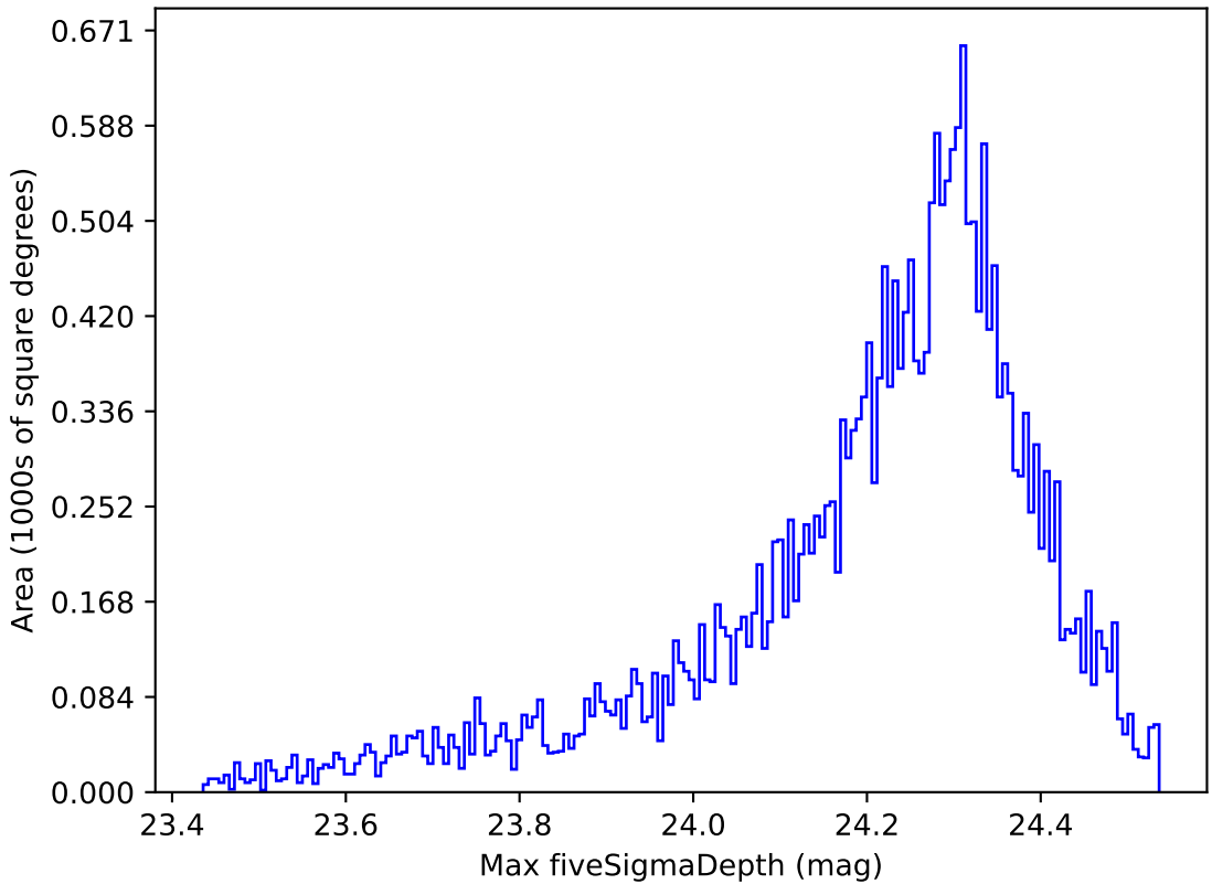
scp_reweight_v3.3_10yrs All sky i band: Max fiveSigmaDepth
