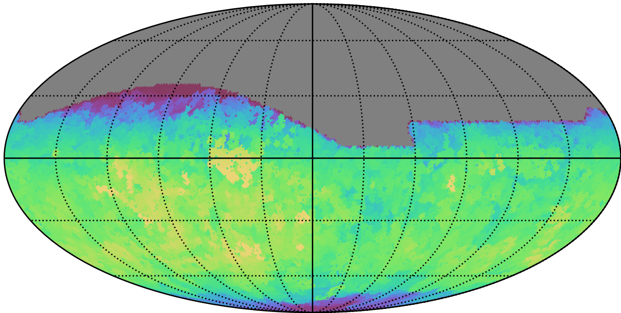
scp_reweight_v3.3_10yrs All sky g band: Max fiveSigmaDepth
