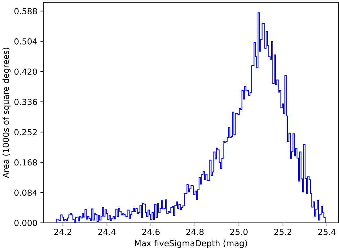
scp_reweight_v3.3_10yrs All sky g band: Max fiveSigmaDepth
