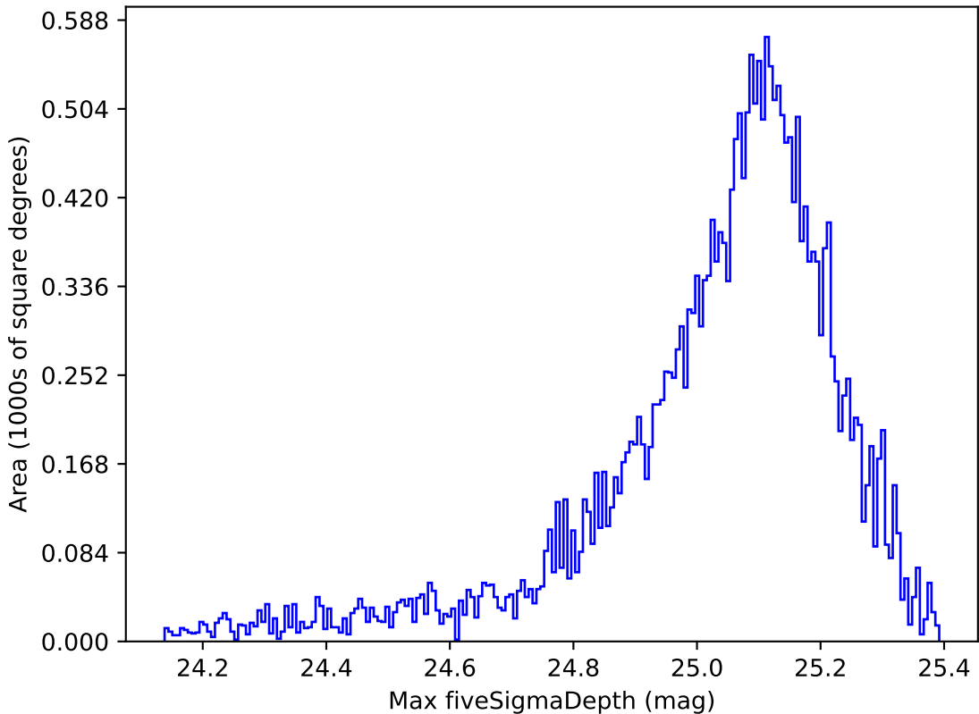
scp_reweight_v3.3_10yrs All sky all bands: Max fiveSigmaDepth
